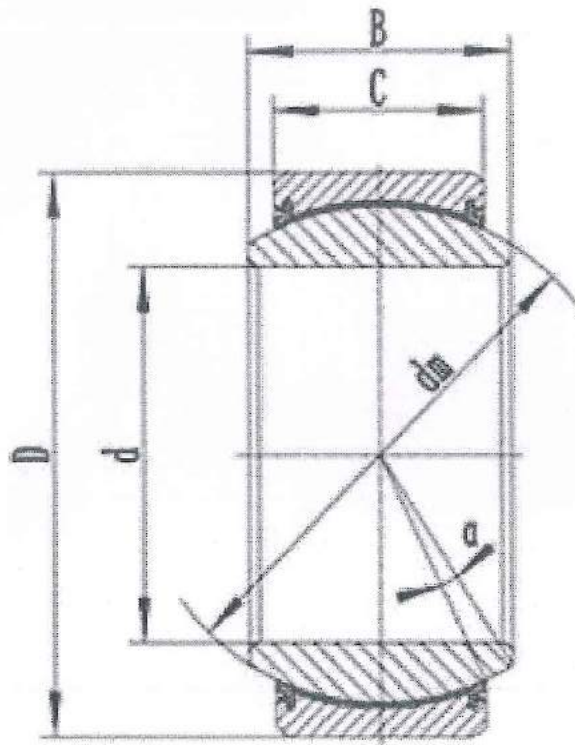
Fig:1 : Typical Cross Sectional view of a Bearing.
